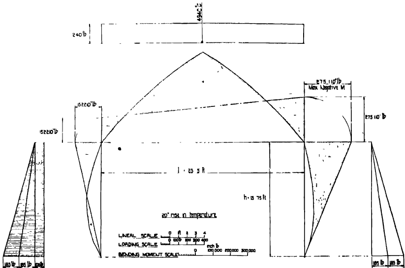
Fig. 118.—Maximum Negative Bending Moment.
